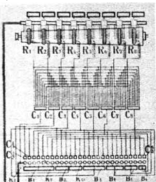
Abb. 3. Compare-Sender
